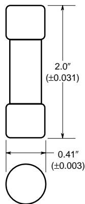
Dimensional Data
