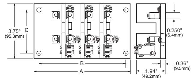
Dimensional Data
