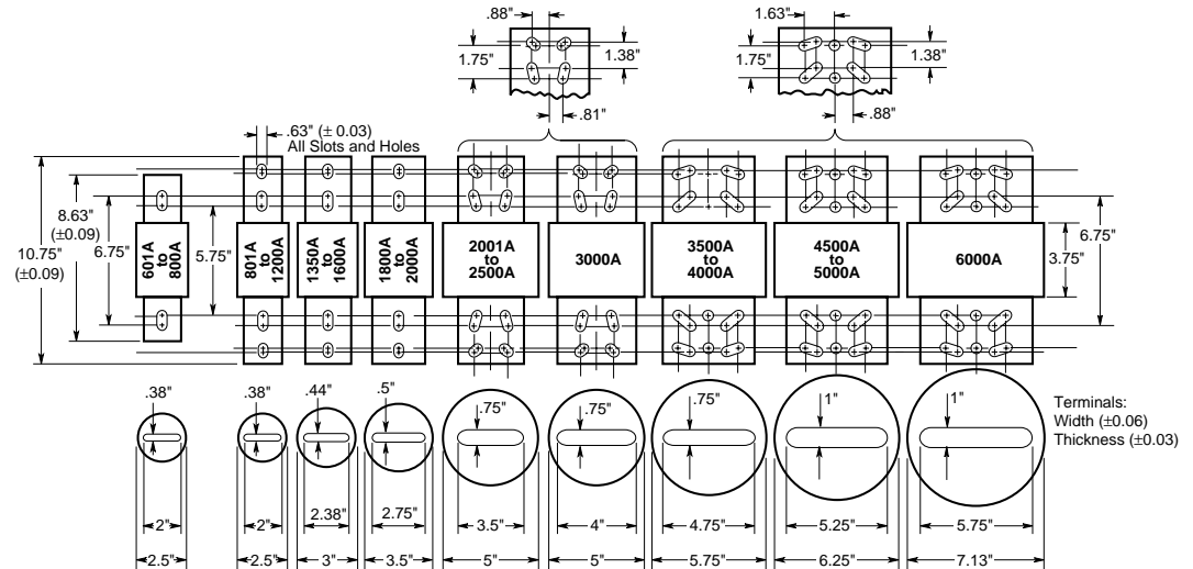
Dimensional Data *All other tolerances (±0.02)
