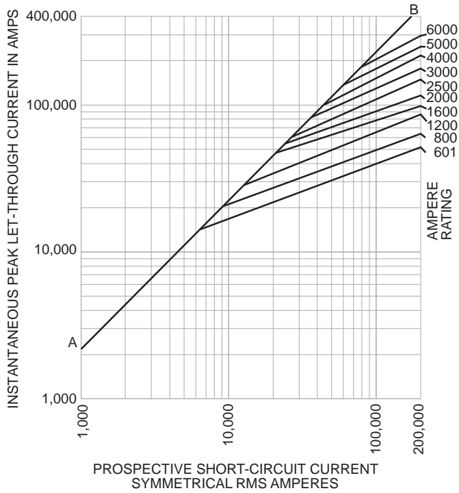
Current-Limitation Curves
