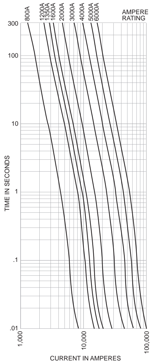
Time-Current Characteristic Curves—Average Melt
